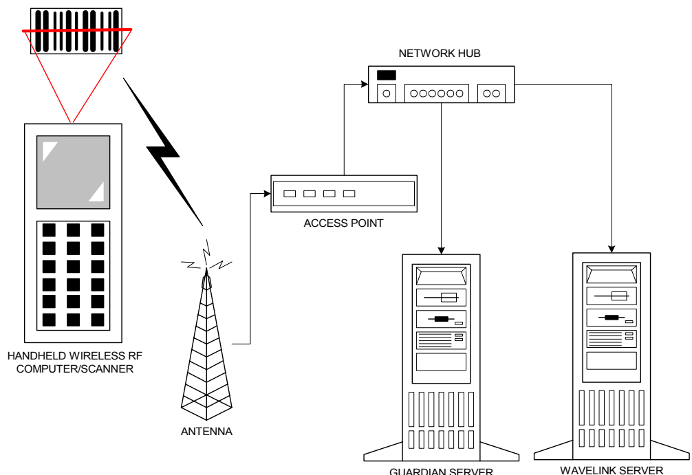
Wireless Warehouse Technical Diagram
