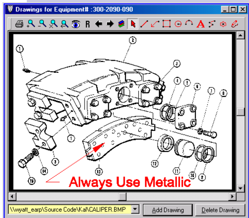
Drawing Screen Showing User Redlining
